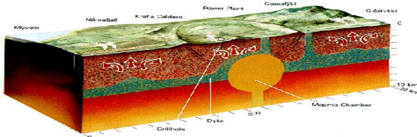
Fig. 14 A block diagram showing schematically the magma body below the Krafla caldera and the dyke formed in the present tectonic episode.
