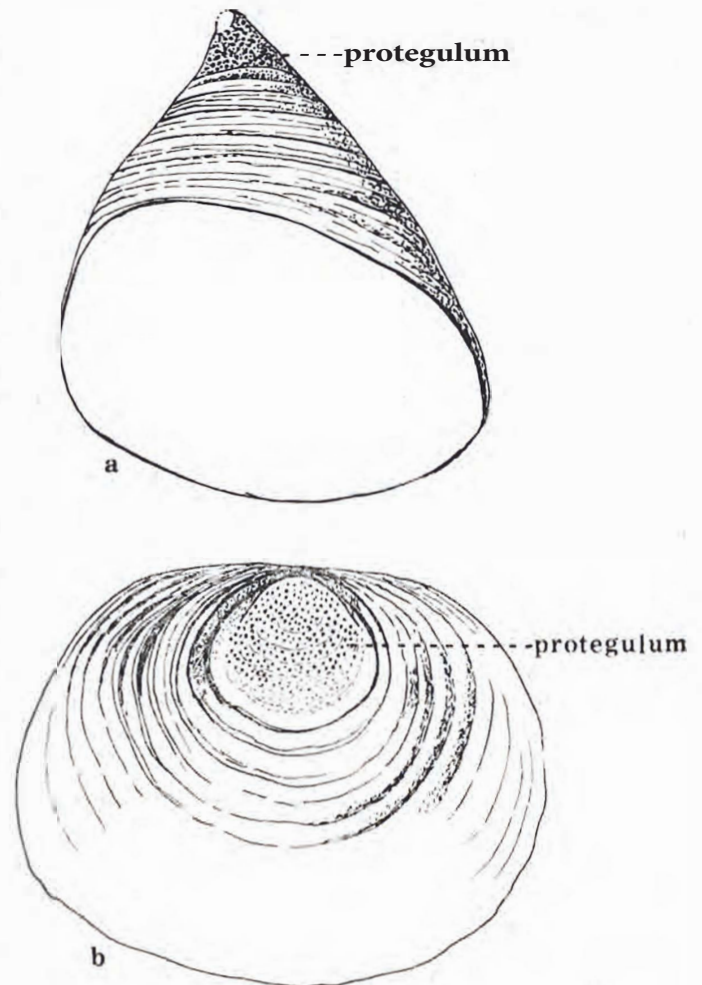
1- Figure 5: Conotreta sp. a) Pedoncular valve, b) Brachial valve.
