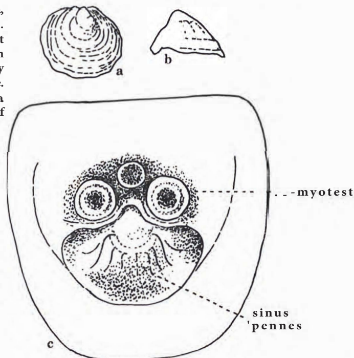
Figure 4: Craniotreta caltepens , nov. gen. nov. sp. Brachial valve. a) Dorsal view, b) Profile, c) Detail from the internal face.
