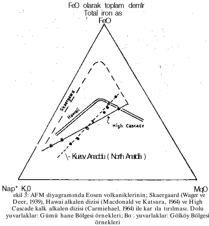
Figure 3: AFM diagram comparing the trend of Eocene volcanics with the trend of Skaergaard (Wager and Deer, 1939) Hawaiian alkaline series (Macdonald and Katsura, 1964) and High Cascade calc alkaline series (Carmichael, 1964). Solid circles: Rocks from Gümü hane; Open circles: Rocks from Gölköy
